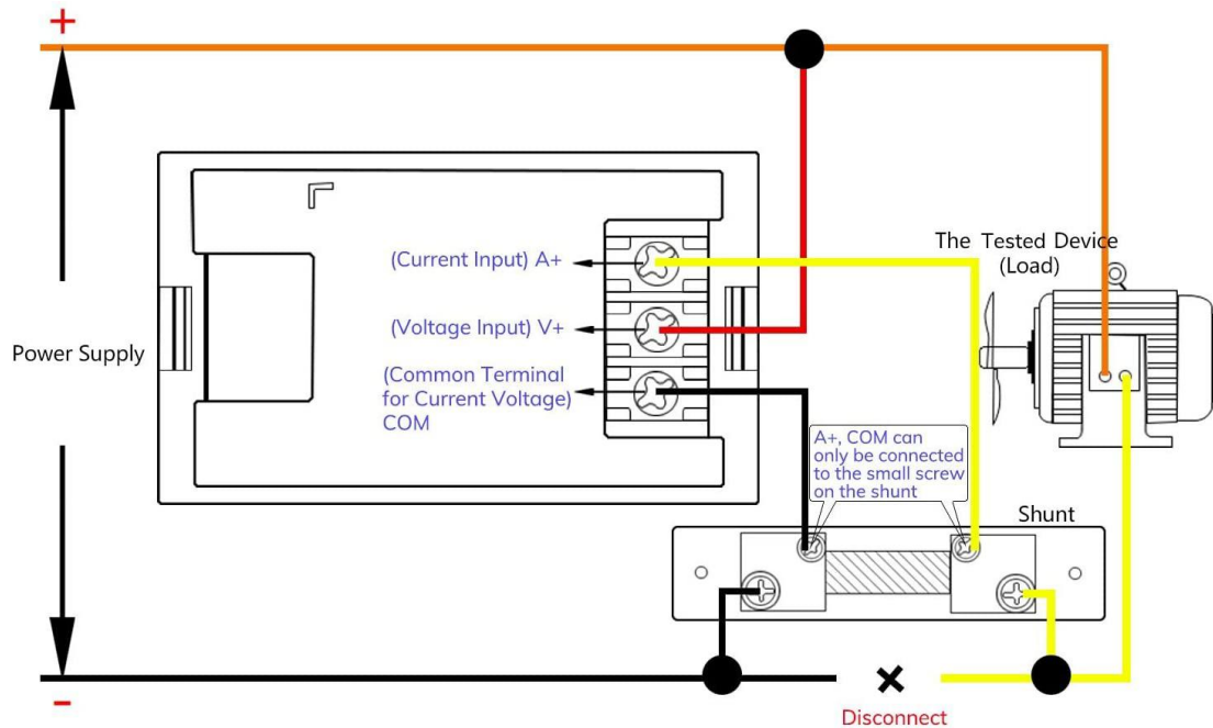
Wiring diagram
